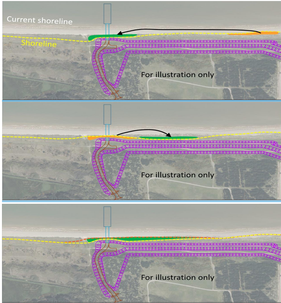
Figure 12: Schematics showing examples of depleted beach sections and the likely mitigation method: beach recycling (top), sediment bypassing (middle) and beach recharge (bottom). The examples assume a net southerly (left to right) longshore drift, but the same principles can be applied in the unlikely event of any period of persistent reversal in the net transport direction. Orange indicates the borrow area and green the deposition area. [Note that the HCDF design shown is indicative only and is known to be outdated, but this does not affect the schematic illustration of beach
